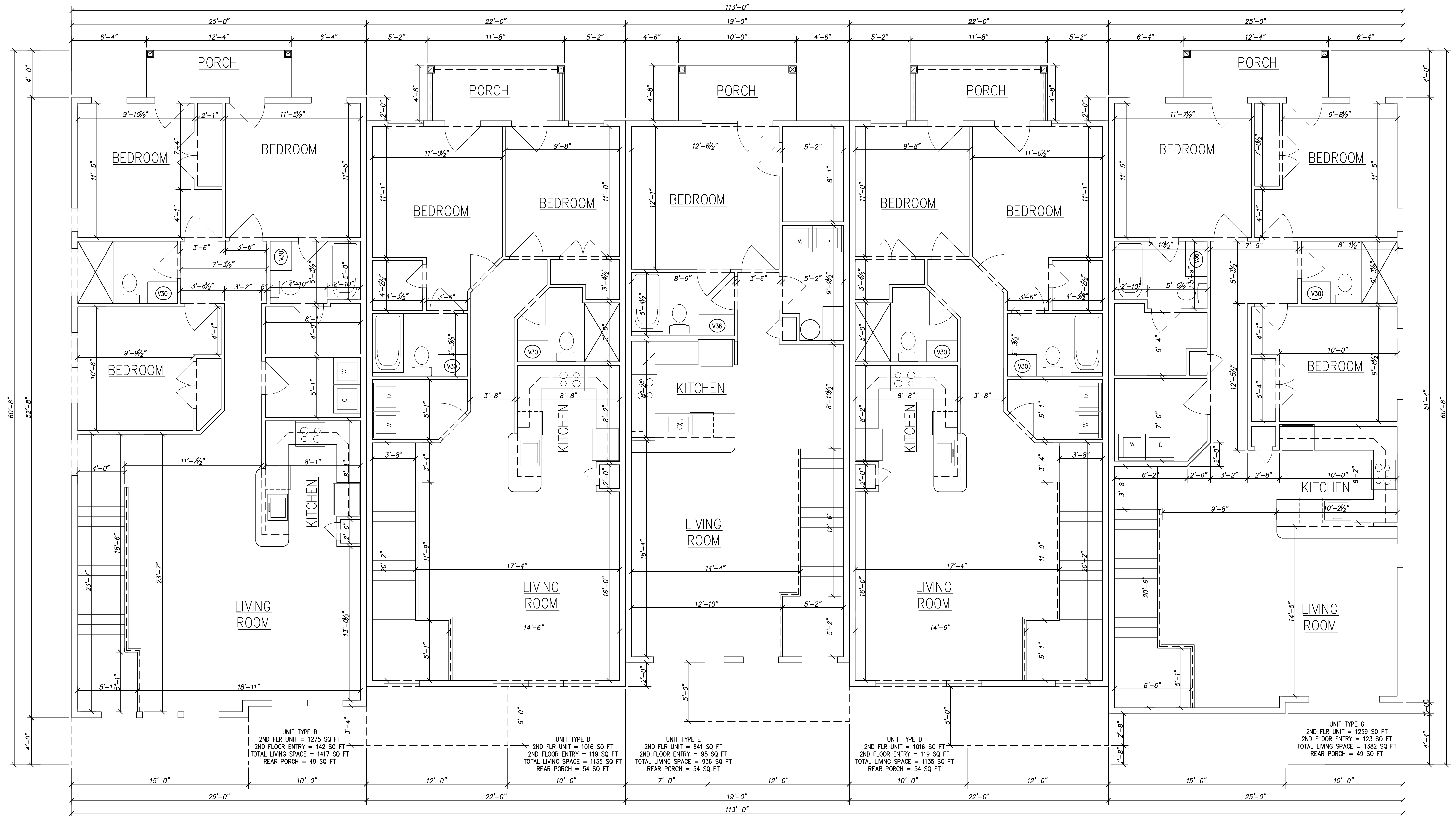
OVERALL 2ND FLOOR PLAN BLDG TYPE A
