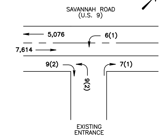
TRAFFIC GENERATION DIAGRAM TRIPS PER DAY (WEEKDAY PEAK HOUR)
